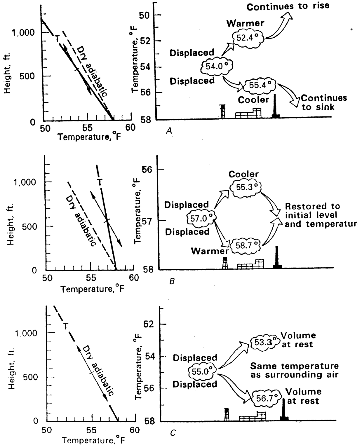
FIGURE 11.5. Effect of atmospheric temperature gradient—or lapse rate—on a displaced volume of air. A. Unstable lapse rate. B. Stable lapse rate. C. Neutral lapse rate. (From Meteorology and Atomic Energy , U.S. AEC, Washington DC, 1955.)
